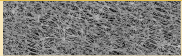
Tetratex PTFE membrane 2000x magnification
